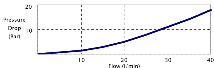
Flow Characteristics
