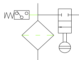
4 Filter, Switch and Fill Valve
