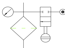
3 Filter, Gauge and Fill Valve
